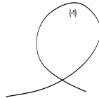
FIGURE 11. \bar{Q} \subset Y(5) is a cycle introduced in the resolution of the cusp
