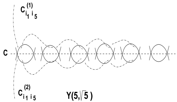
FIGURE 16. Curves C_{i_1, \dots, i_5}^{(1)} and C_{i_1, \dots, i_5}^{(2)} are pre-images of \bar{C}_{i_1, \dots, i_5}
