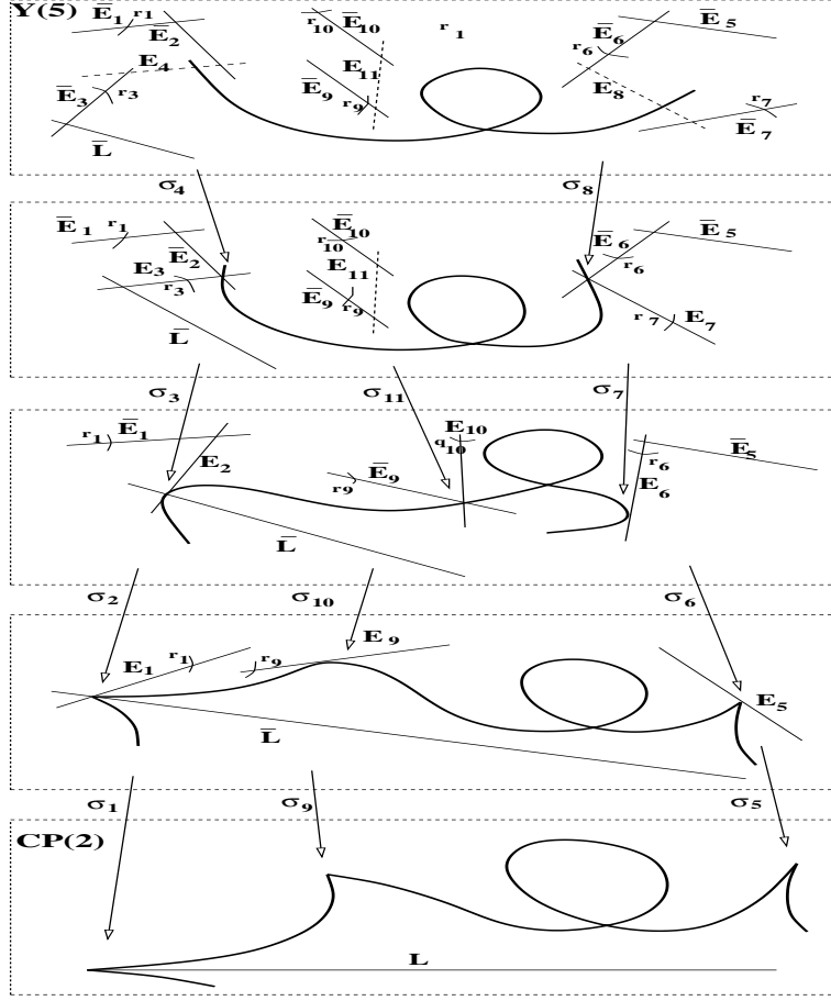
FIGURE 18. Resolution of H_3 .
