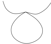
FIGURE 14. Double cusps of Klein degree 10 curve at the points v_i, i = 11, \dots, 16
