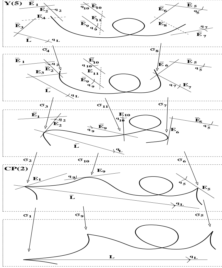
FIGURE 17. Resolution of \mathcal{H}_2
