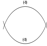
FIGURE 12. Cycles composed by two components on Y(5, (\sqrt{5}))
