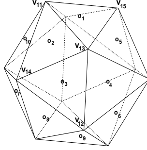
FIGURE 5. Vertices and centers of faces of an icosahedron
