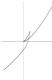
FIGURE 3. A cuspidal quintic curve and the line at infinity are the tangency set of \mathcal{H}_2 and \mathcal{H}_3
