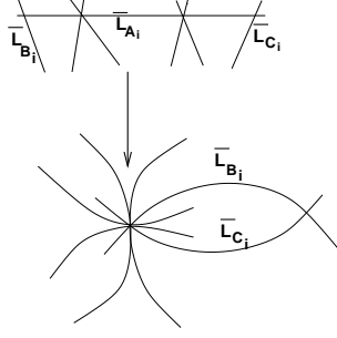
FIGURE 8. Contraction producing the point r_{A_i} of \mathbb{P}_{\mathbb{C}}^1 \times \mathbb{P}_{\mathbb{C}}^1
