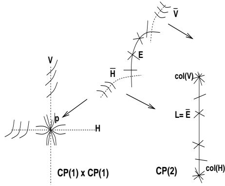
FIGURE 9. Passing from \mathbb{P}_{\mathbb{C}}^1 \times \mathbb{P}_{\mathbb{C}}^1 to \mathbb{P}^2 .
