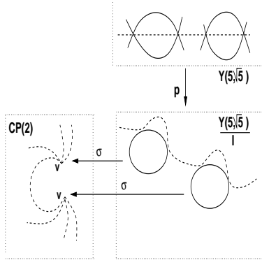
FIGURE 15. The 2-fold covering of Y(5, (\sqrt{5})) over the blown up plane
