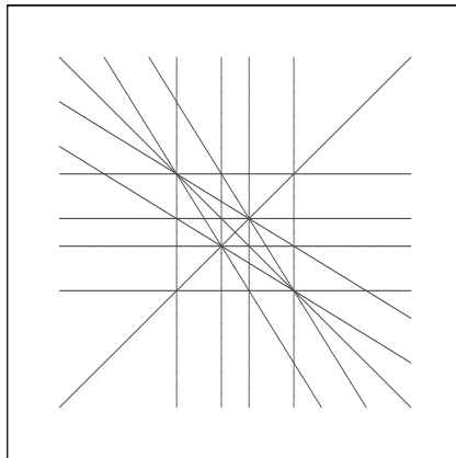
FIGURE 1. Real picture of the arrangement of lines invariant by \mathcal{H}_5 and \mathcal{H}_9 . The line at infinity is also invariant, besides the 14 lines in the configuration.
