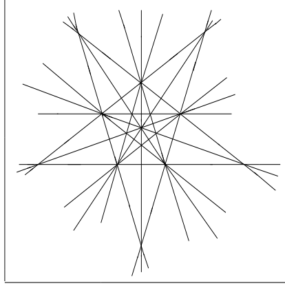
FIGURE 6. The Icosahedral configuration of lines
