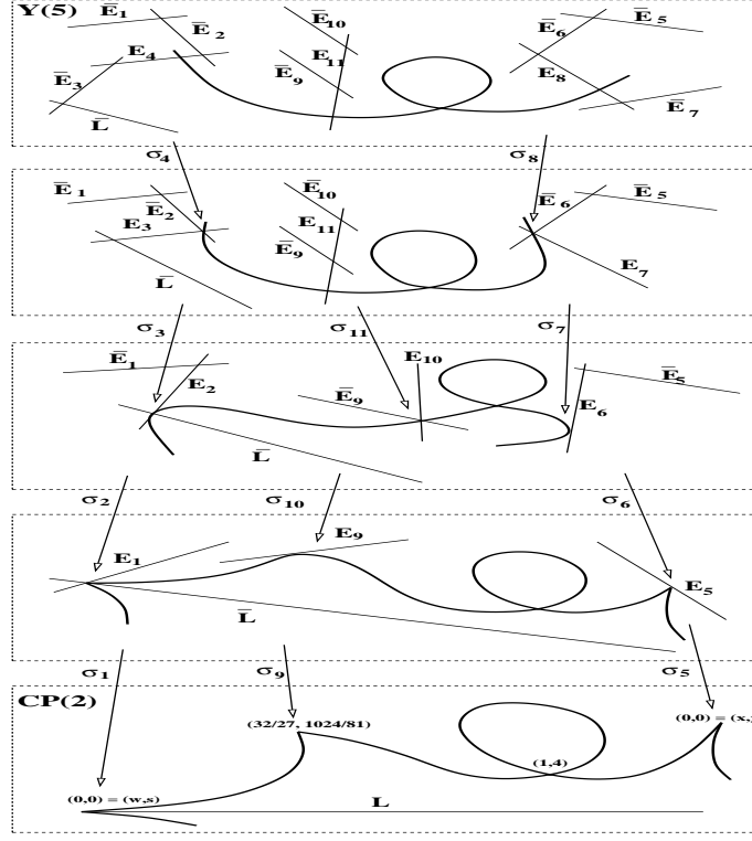
FIGURE 10. The 11 blow ups composing f : Y(5) \rightarrow \mathbb{P}^2 .
