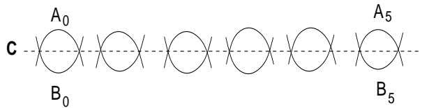
FIGURE 13. The resolution of cusps of Y(5, (\sqrt{5}))
