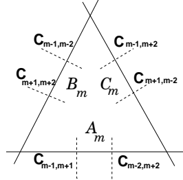
FIGURE 4. Intersections between diagonals C_{ij} and cycles, with integers taken modulo 5.
