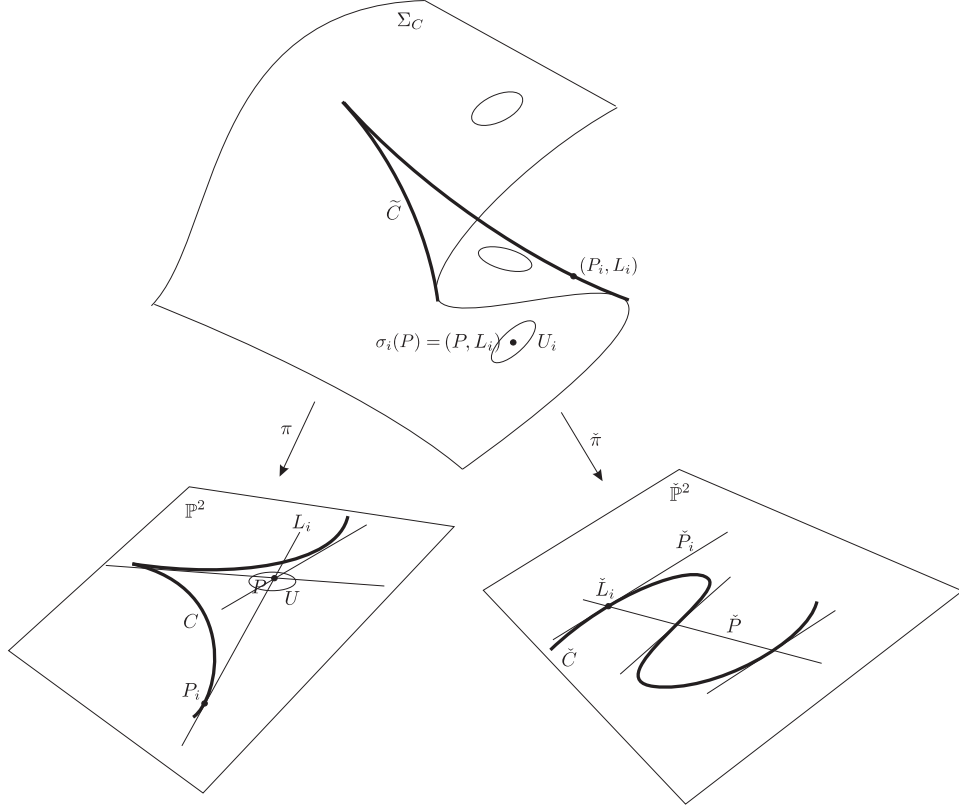
FIGURE 1. The algebraic web \text{Leg } C
