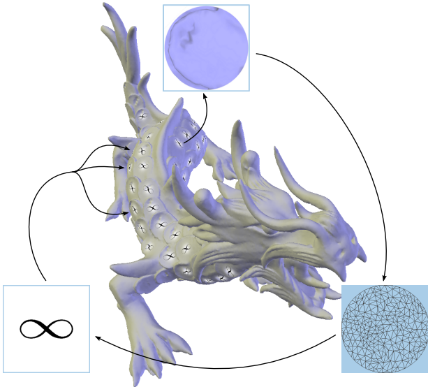
Figure 7: SAMPLE application: mesh parameterization. One of the dragon scales is elected to be the exemplar region (top); the exemplar is parameterized using a standard procedure (bottom right); the infinity logo image (bottom left) is used to texture the similar dragon scales seamlessly.
