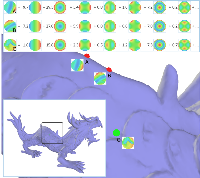
Figure 3: Zernike expansions for heightmaps. Only the magnitudes of the complex values for the coefficients (top three row numbers) and Zernike polynomials (images after the equal signs) are shown. Although vertices A and B (in red) are similar, their heightmaps have improper alignment based on principal directions. By converting them to Zernike coefficients, the heightmaps are correctly compared. Vertex C (in green) is also correctly classified as different than vertices A and B.
