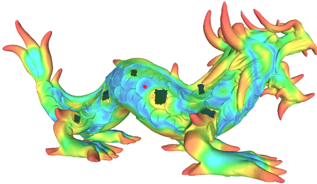
Figure 14: Test of our feature space using the Asian Dragon model with holes and inconsistencies. While the dragon scales with holes are classified as different than the selected scale, the other scales remain correctly classified.
