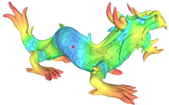
Figure 13: Feature space using HKS. The colors show the Euclidean differences between the HKS of the selected vertex (in red) and all other vertices, considering the time parameter t of the heat-diffusion process to be in range [12, 32] over the same sampled scale of the original paper [6]. The difference increases as the color changes from blue to green to red.
