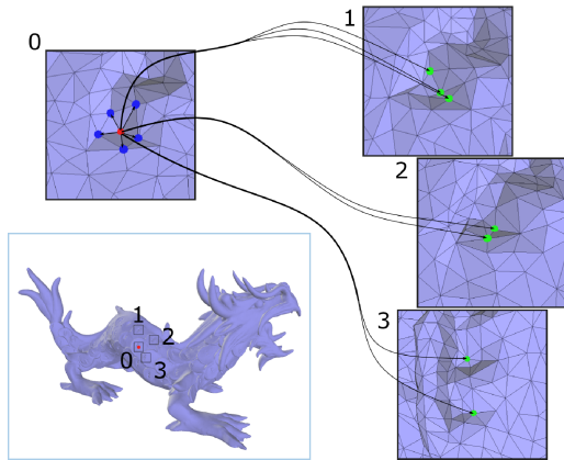
Figure 6: Illustration of the geometry and feature spaces. Several geometry neighbours of the selected vertex (in red) on a dragon scale are shown in blue (box 0). While some of the feature neighbours are shown in green (boxes 1, 2 and 3).
